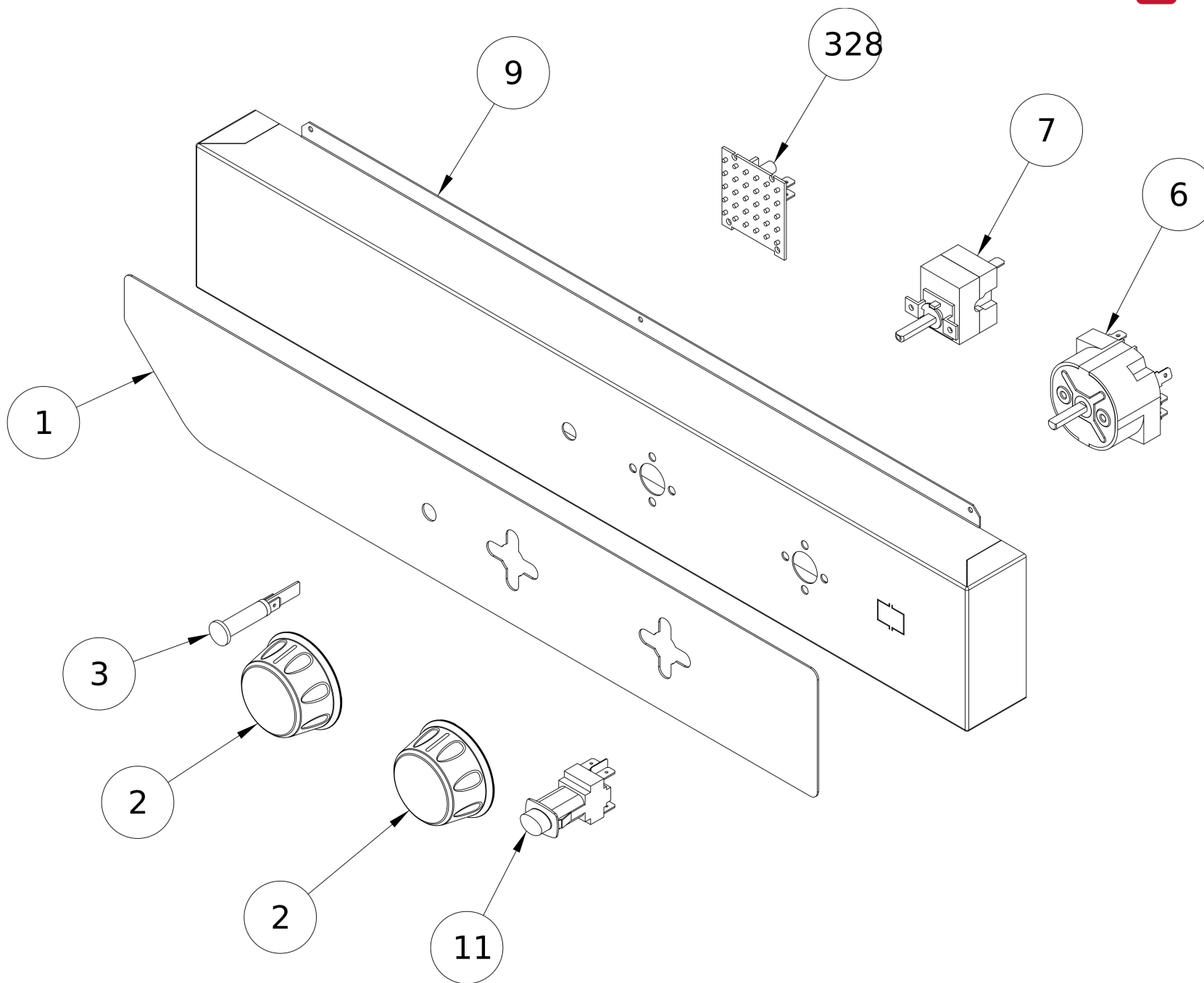
Frontal panel
