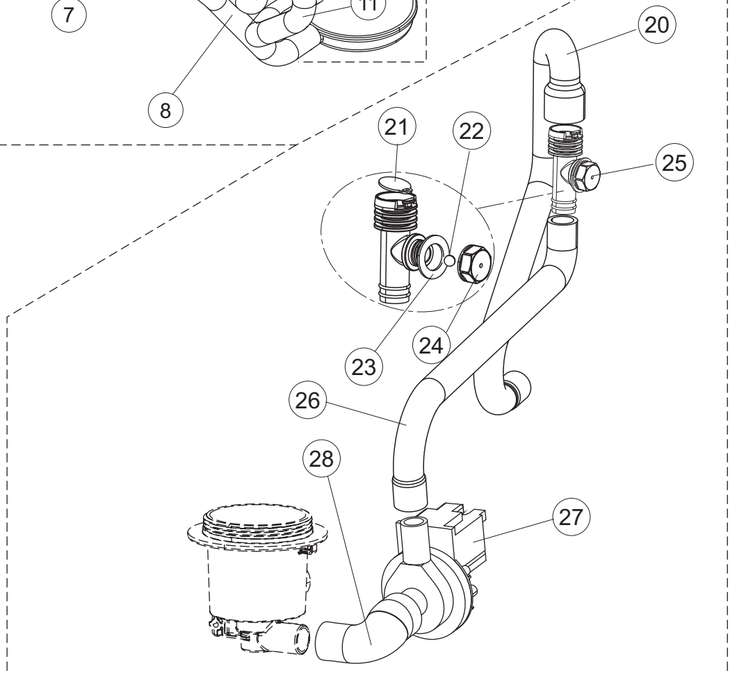
Drain pump
